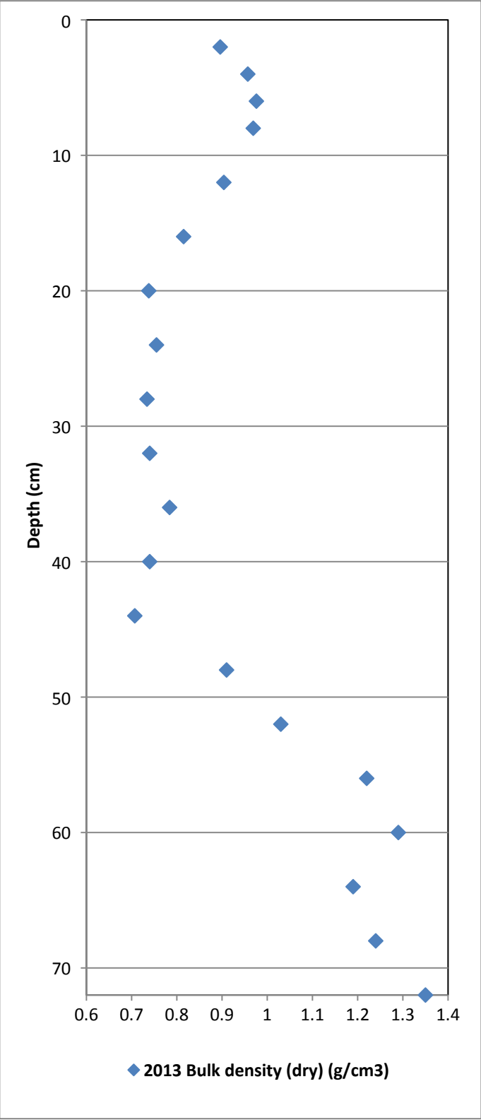
Figure 26. Vertical Profiles of Bulk Density and COCs for Core OA26 First MNR Report Palos Verdes Shelf (OU 5 of the Montrose Chemical Corp. Superfund Site) Los Angeles County, California
