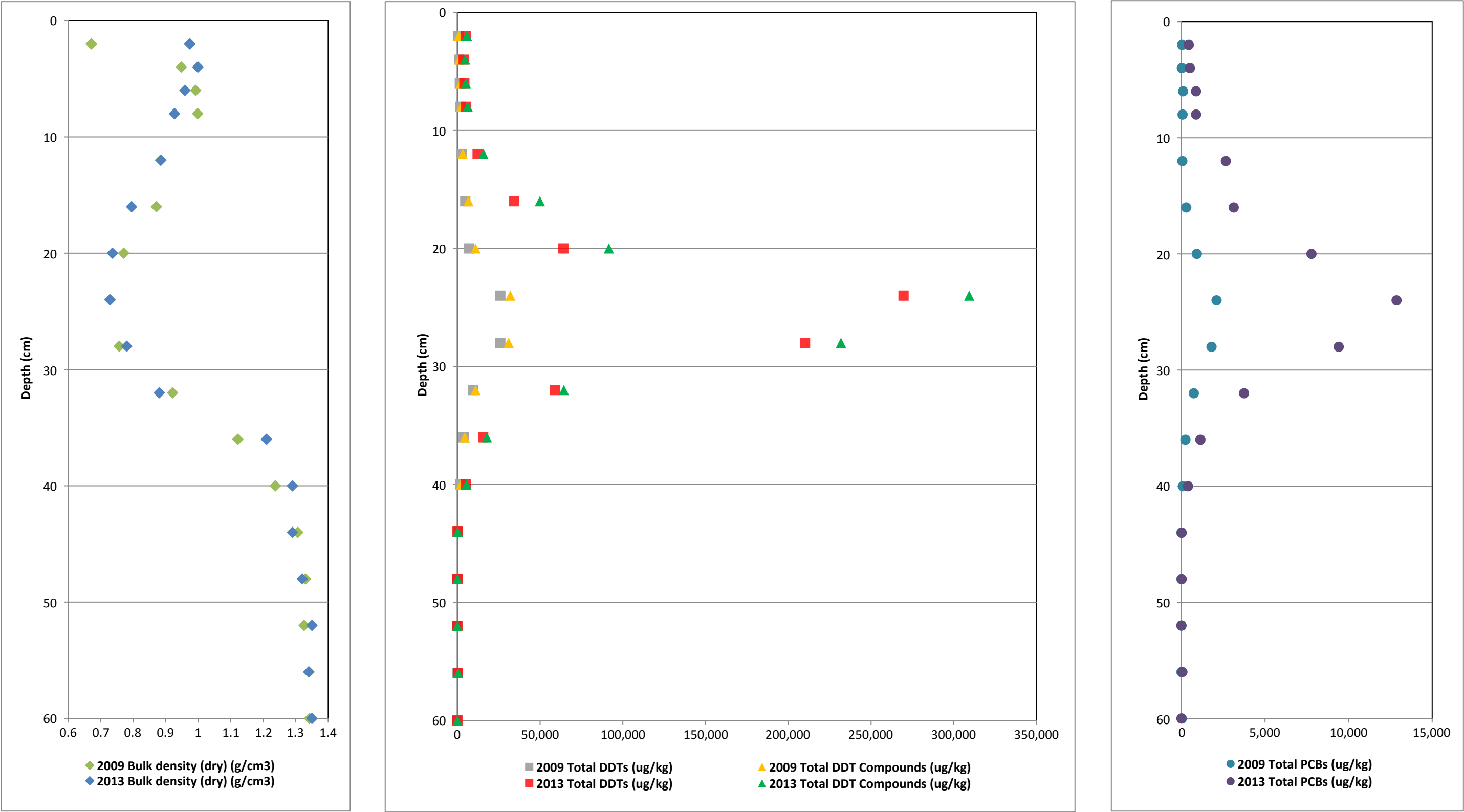
Figure 3. Vertical Profiles of Bulk Density and COCs for Core OA03 First MNR Report Palos Verdes Shelf (OU 5 of the Montrose Chemical Corp. Superfund Site) Los Angeles County, California
