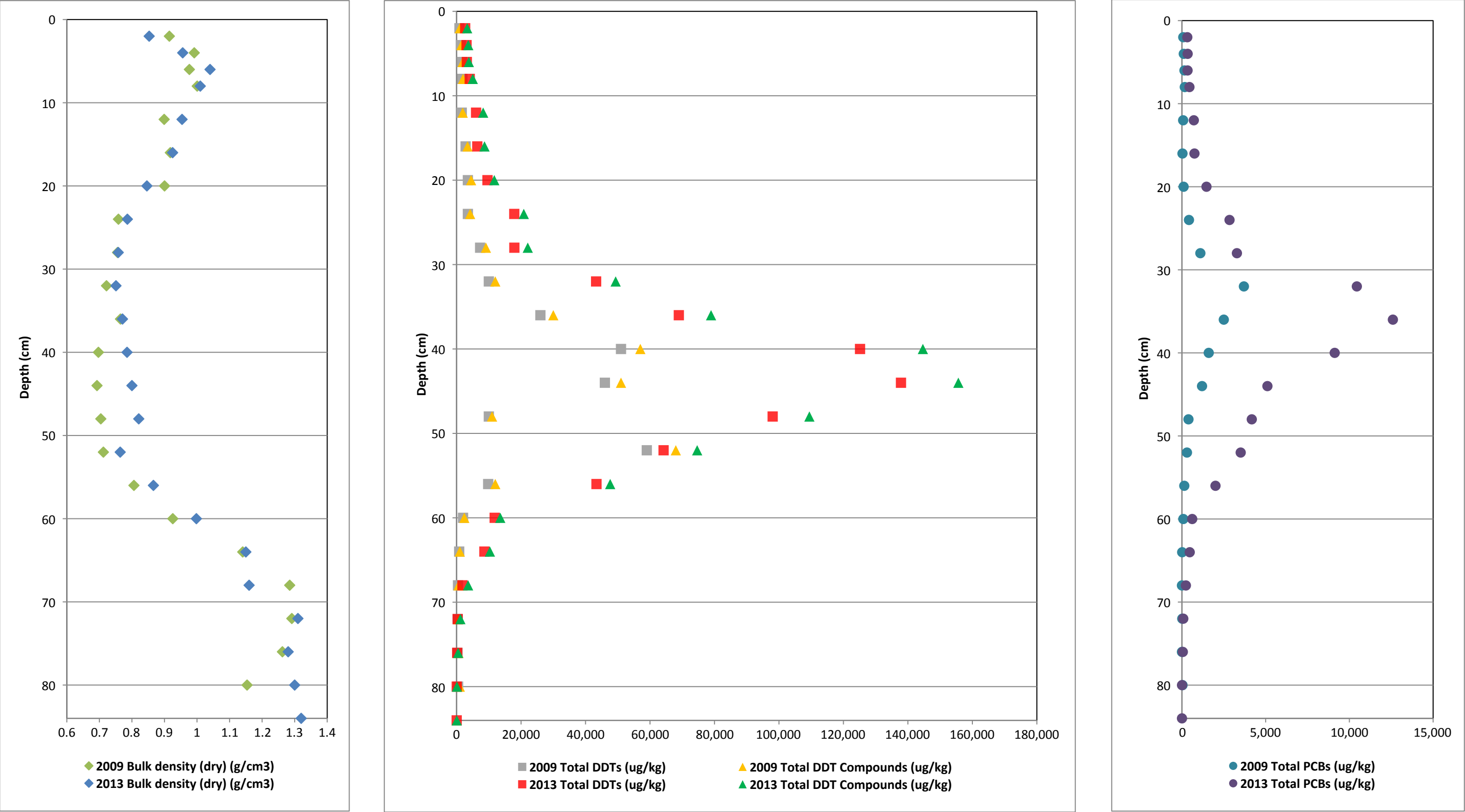
Figure 5. Vertical Profiles of Bulk Density and COCs for Core OA05 First MNR Report Palos Verdes Shelf (OU 5 of the Montrose Chemical Corp. Superfund Site) Los Angeles County, California
