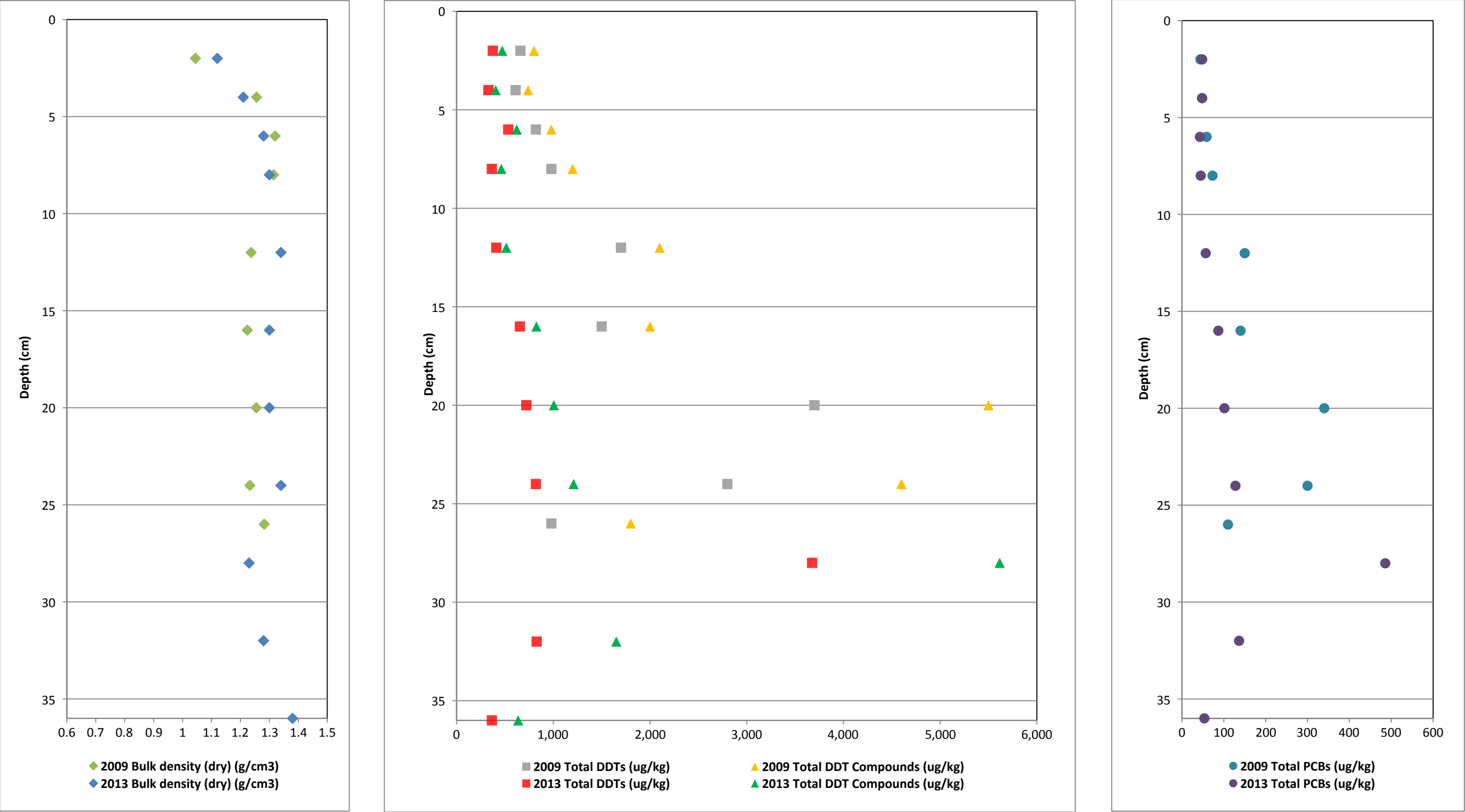
Figure 25. Vertical Profiles of Bulk Density and COCs for Core OA25 First MNR Report Palos Verdes Shelf (OU 5 of the Montrose Chemical Corp. Superfund Site) Los Angeles County, California
