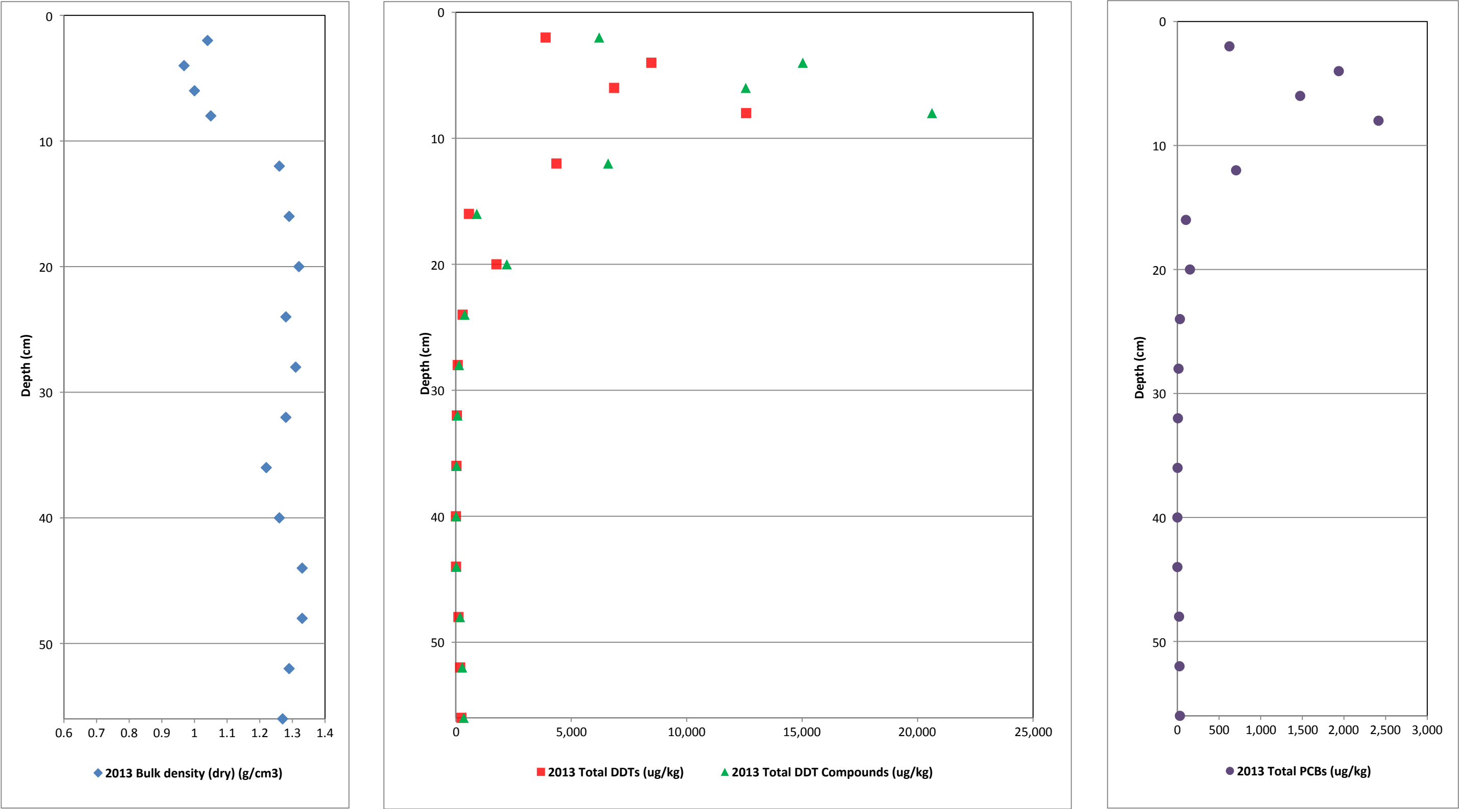
Figure 35. Vertical Profiles of Bulk Density and COCs for Core OA35 First MNR Report Palos Verdes Shelf (OU 5 of the Montrose Chemical Corp. Superfund Site) Los Angeles County, California
