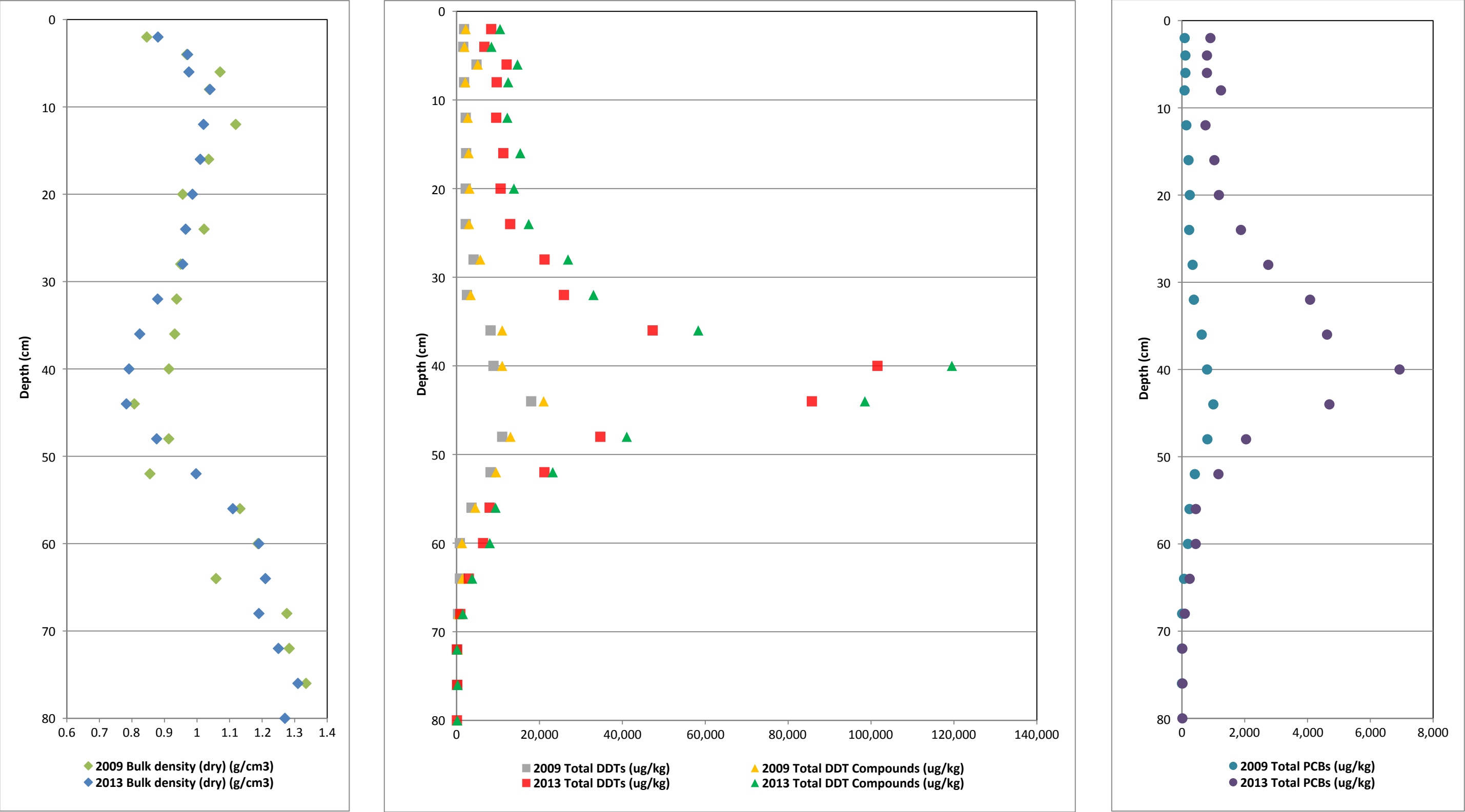
Figure 8. Vertical Profiles of Bulk Density and COCs for Core OA08 First MNR Report Palos Verdes Shelf (OU 5 of the Montrose Chemical Corp. Superfund Site) Los Angeles County, California
