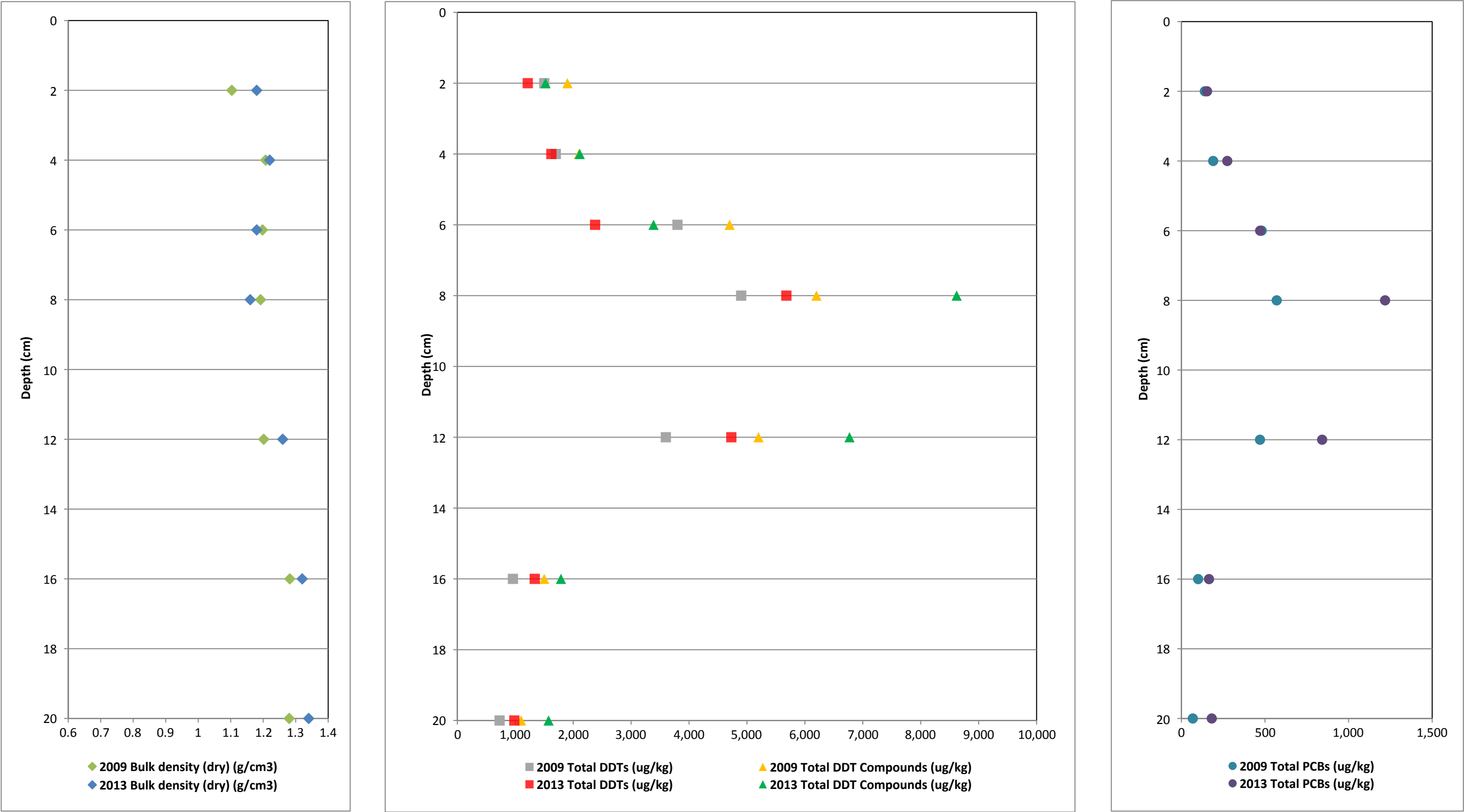
Figure 24. Vertical Profiles of Bulk Density and COCs for Core OA24 First MNR Report Palos Verdes Shelf (OU 5 of the Montrose Chemical Corp. Superfund Site) Los Angeles County, California
