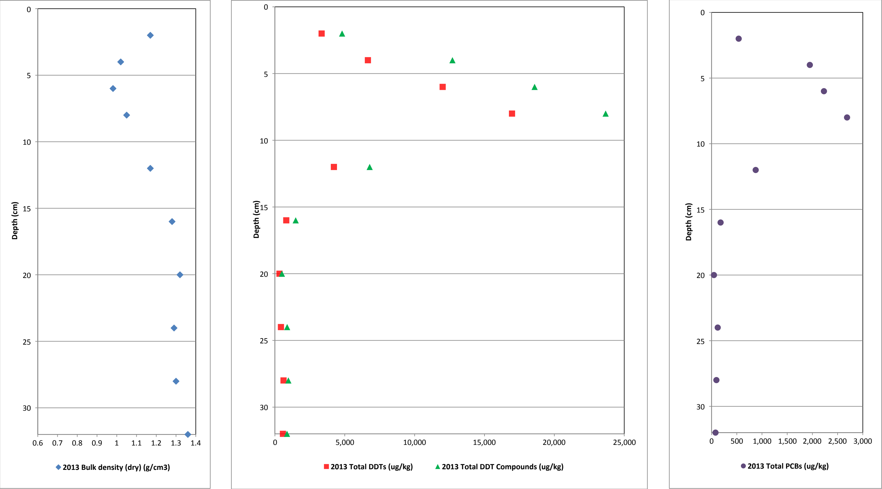
Figure 34. Vertical Profiles of Bulk Density and COCs for Core OA34 First MNR Report Palos Verdes Shelf (OU 5 of the Montrose Chemical Corp. Superfund Site) Los Angeles County, California
