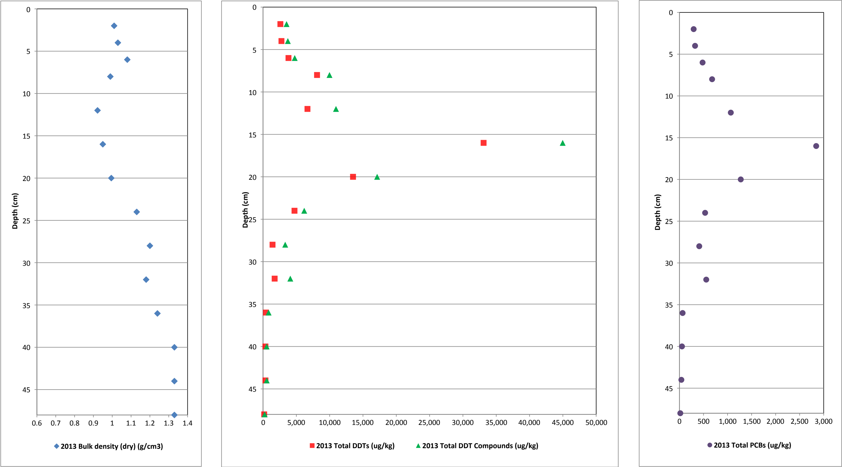
Figure 32. Vertical Profiles of Bulk Density and COCs for Core OA32 First MNR Report Palos Verdes Shelf (OU 5 of the Montrose Chemical Corp. Superfund Site) Los Angeles County, California
