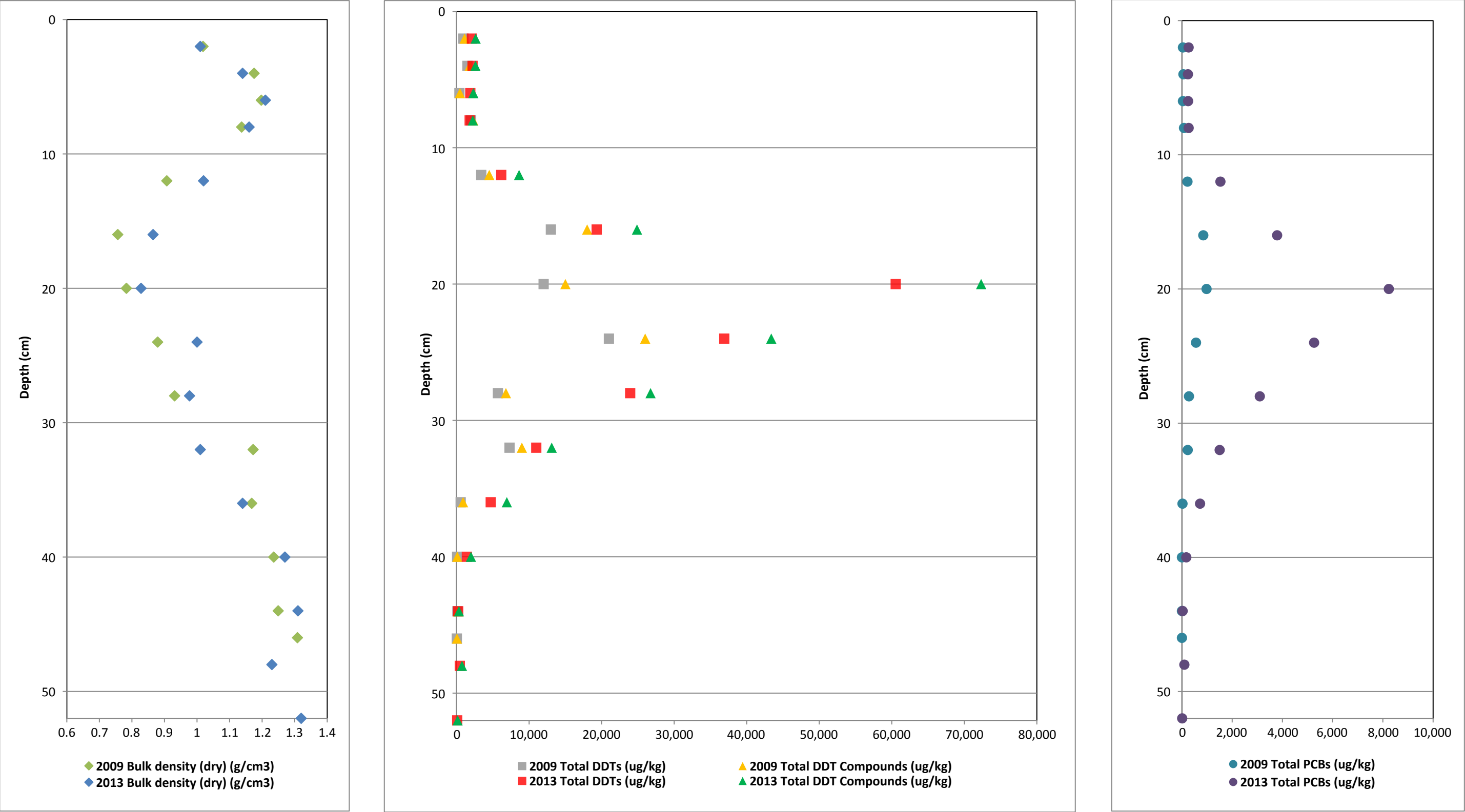
Figure 13. Vertical Profiles of Bulk Density and COCs for Core OA13 First MNR Report Palos Verdes Shelf (OU 5 of the Montrose Chemical Corp. Superfund Site) Los Angeles County, California
