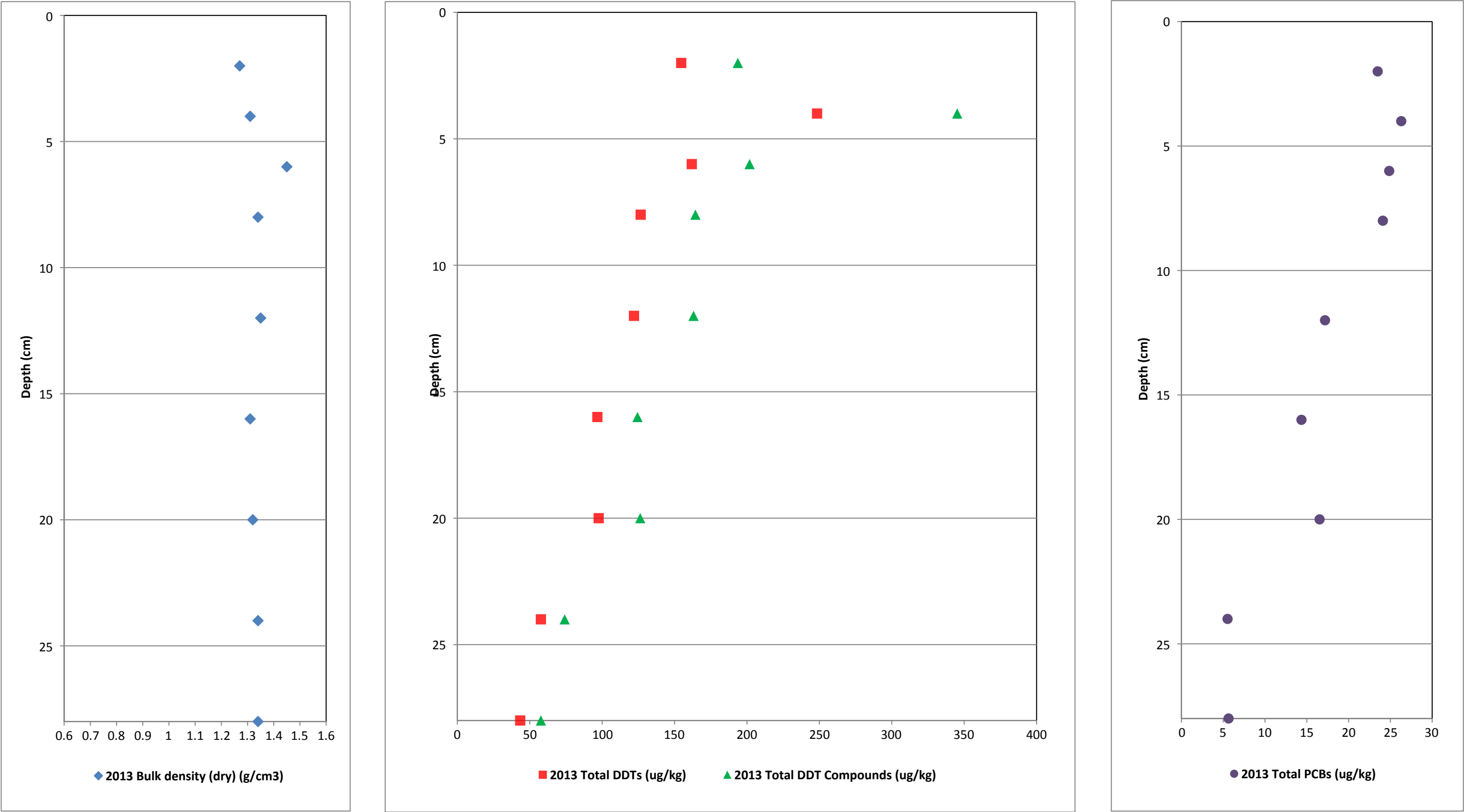
Figure 33. Vertical Profiles of Bulk Density and COCs for Core OA33 First MNR Report Palos Verdes Shelf (OU 5 of the Montrose Chemical Corp. Superfund Site) Los Angeles County, California
