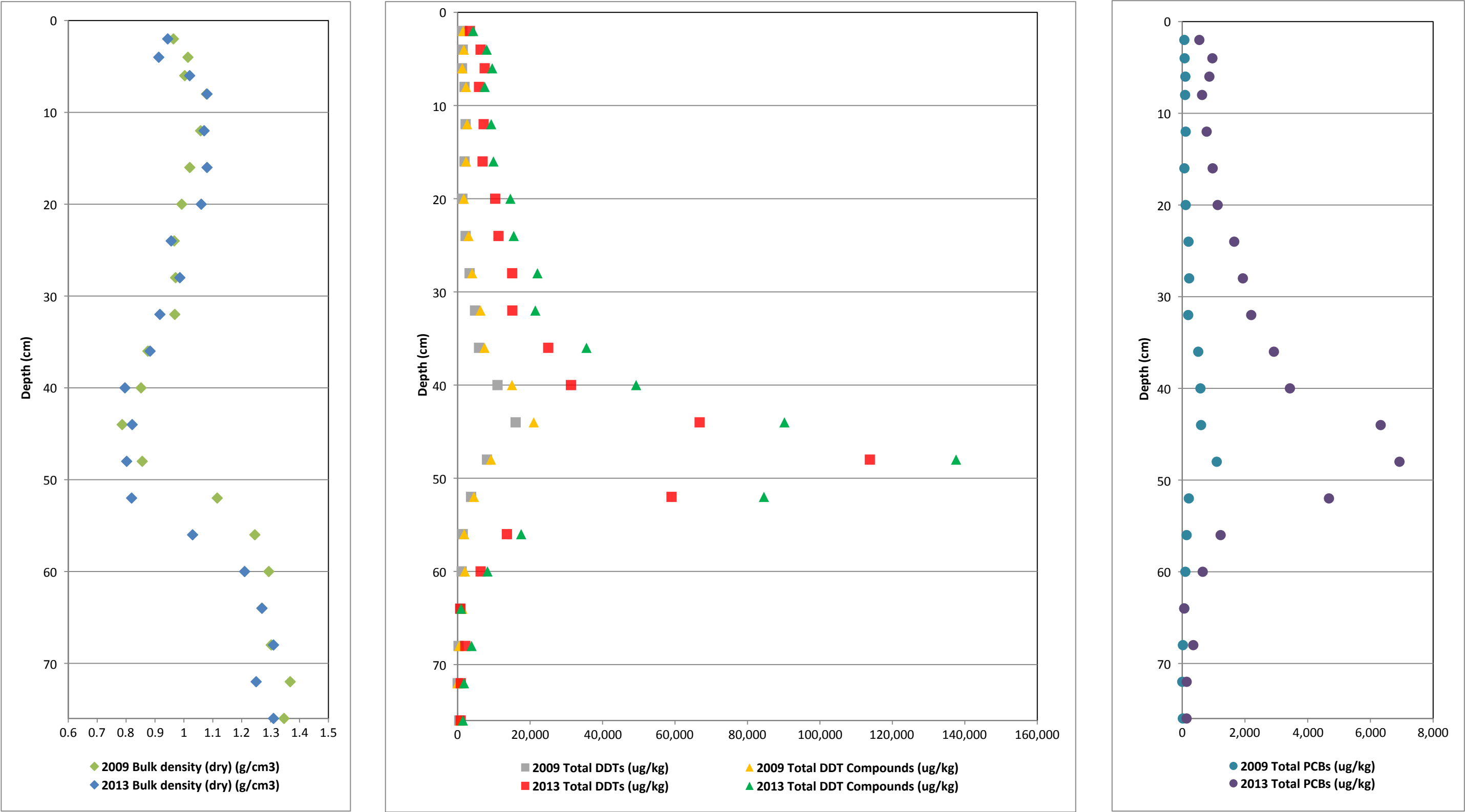
Figure 6. Vertical Profiles of Bulk Density and COCs for Core OA06 First MNR Report Palos Verdes Shelf (OU 5 of the Montrose Chemical Corp. Superfund Site) Los Angeles County, California
