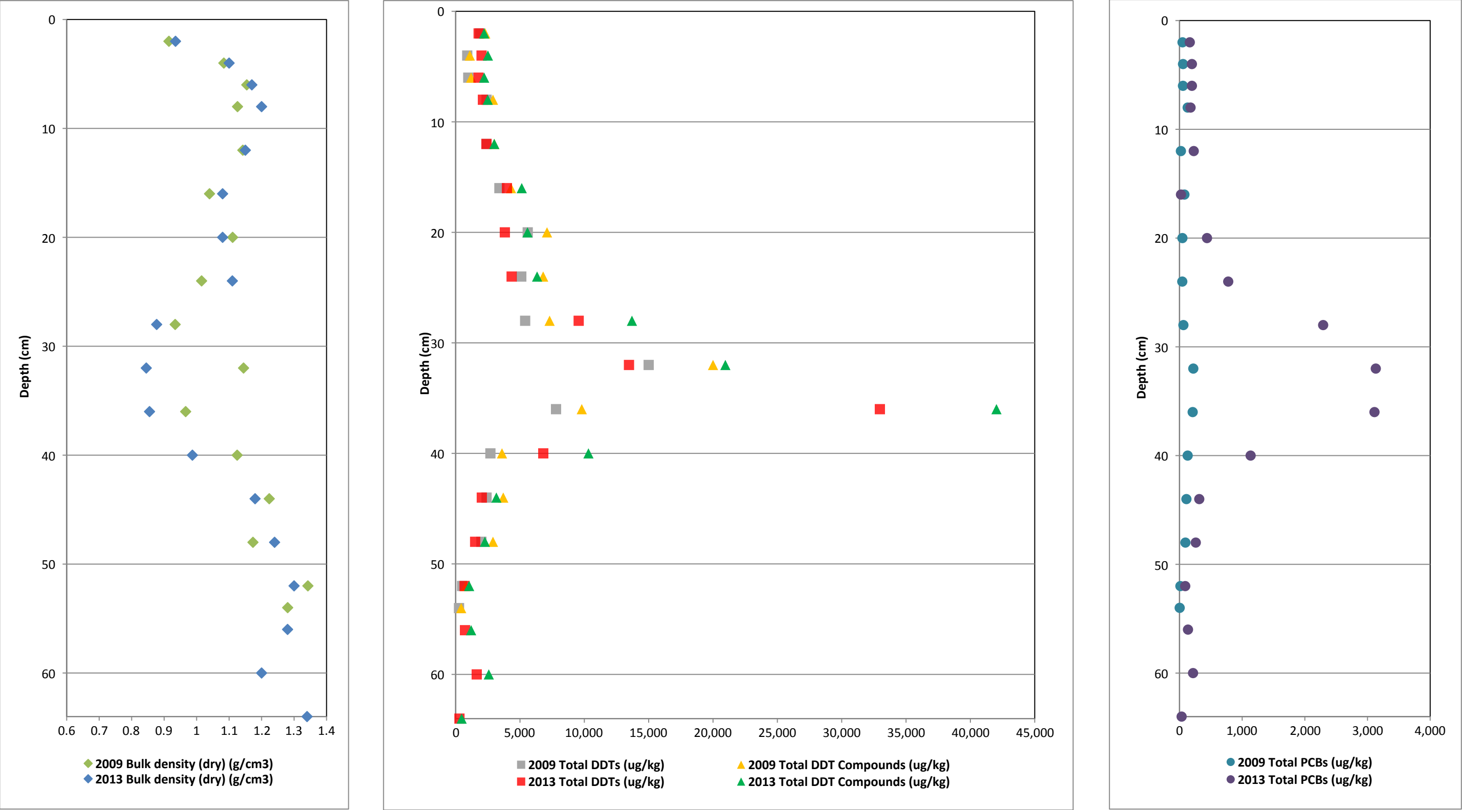
Figure 14. Vertical Profiles of Bulk Density and COCs for Core OA14 First MNR Report Palos Verdes Shelf (OU 5 of the Montrose Chemical Corp. Superfund Site) Los Angeles County, California
