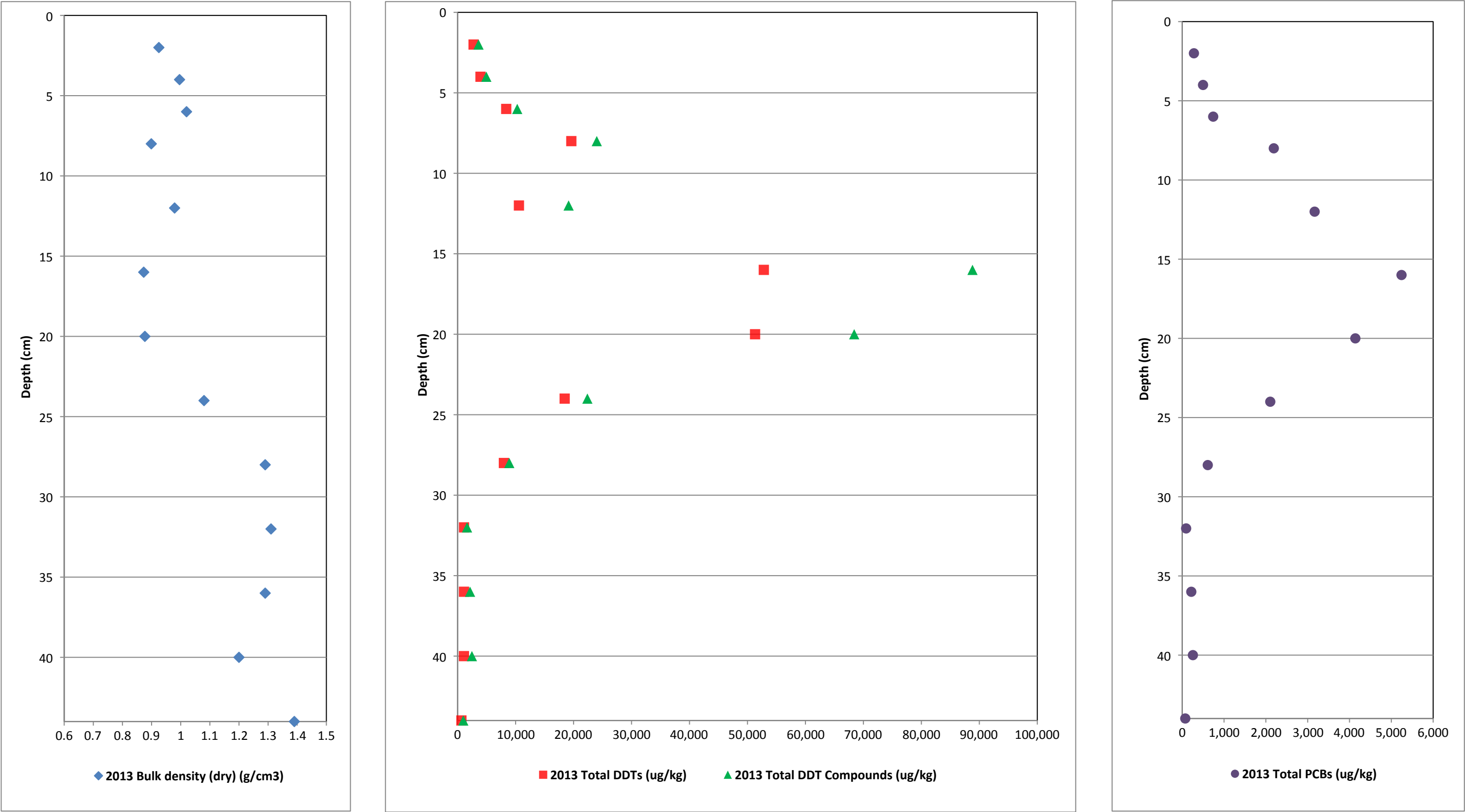
Figure 28. Vertical Profiles of Bulk Density and COCs for Core OA28 First MNR Report Palos Verdes Shelf (OU 5 of the Montrose Chemical Corp. Superfund Site) Los Angeles County, California
