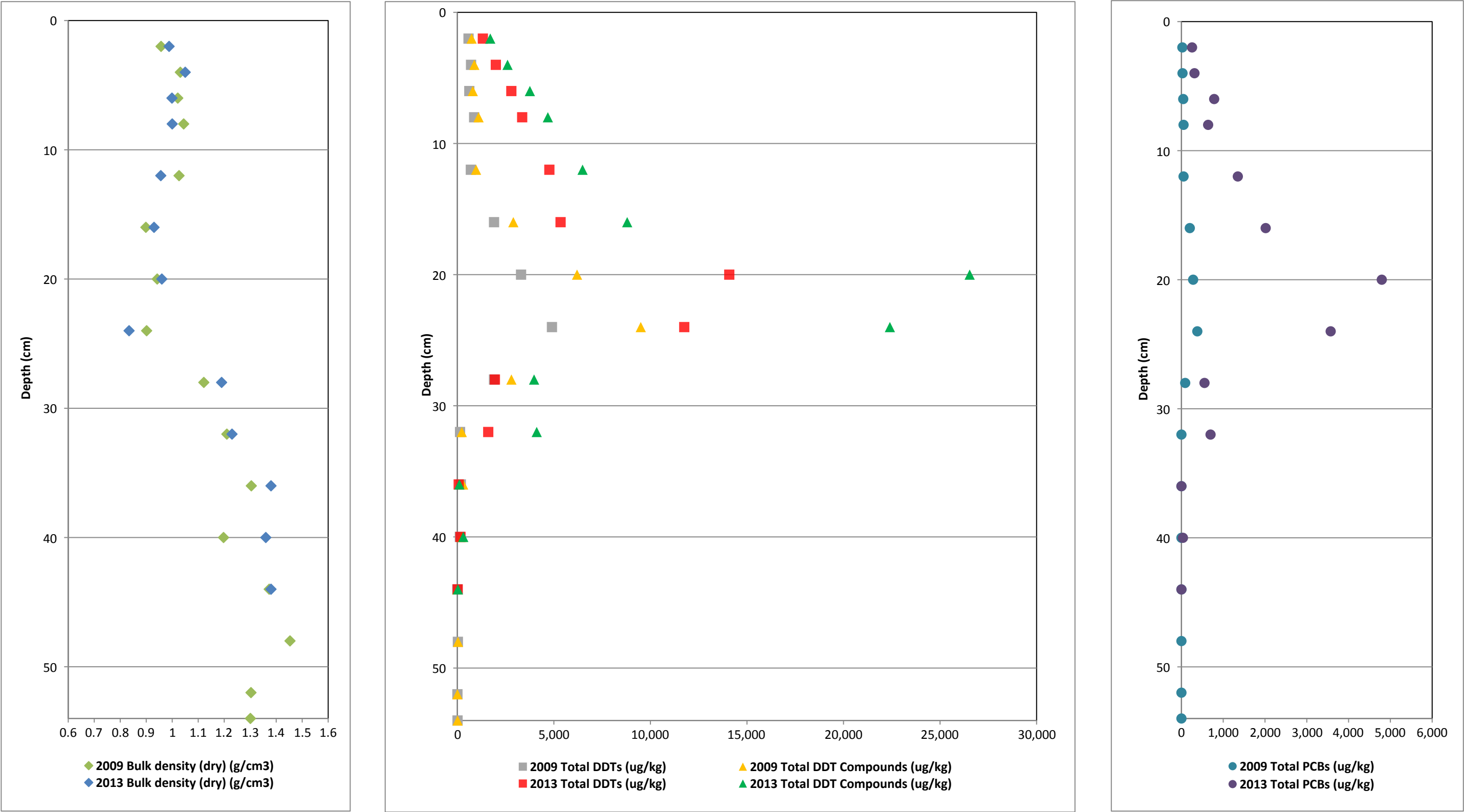
Figure 18. Vertical Profiles of Bulk Density and COCs for Core OA18 First MNR Report Palos Verdes Shelf (OU 5 of the Montrose Chemical Corp. Superfund Site) Los Angeles County, California
