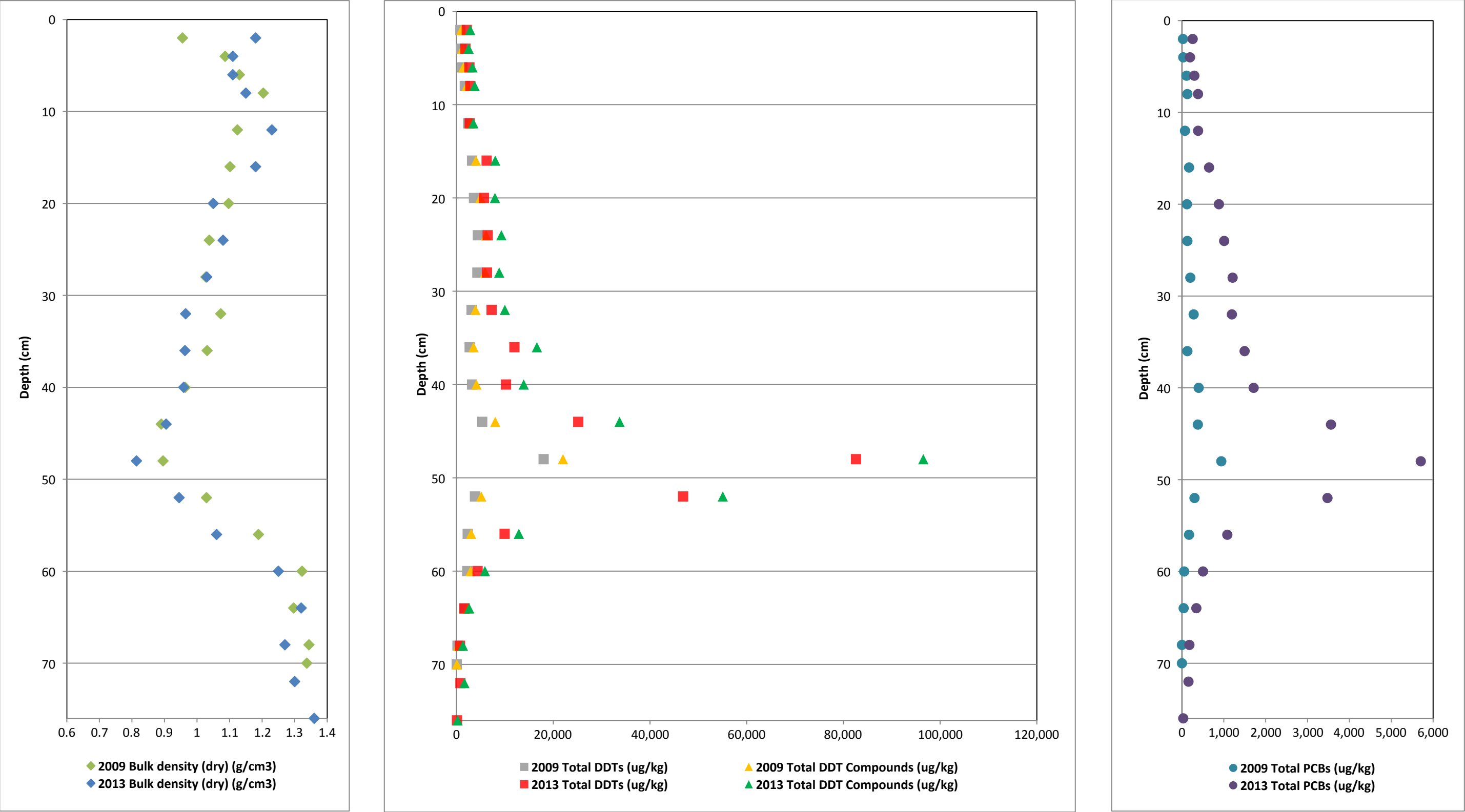
Figure 2. Vertical Profiles of Bulk Density and COCs for Core OA02 First MNR Report Palos Verdes Shelf (OU 5 of the Montrose Chemical Corp. Superfund Site) Los Angeles County, California
