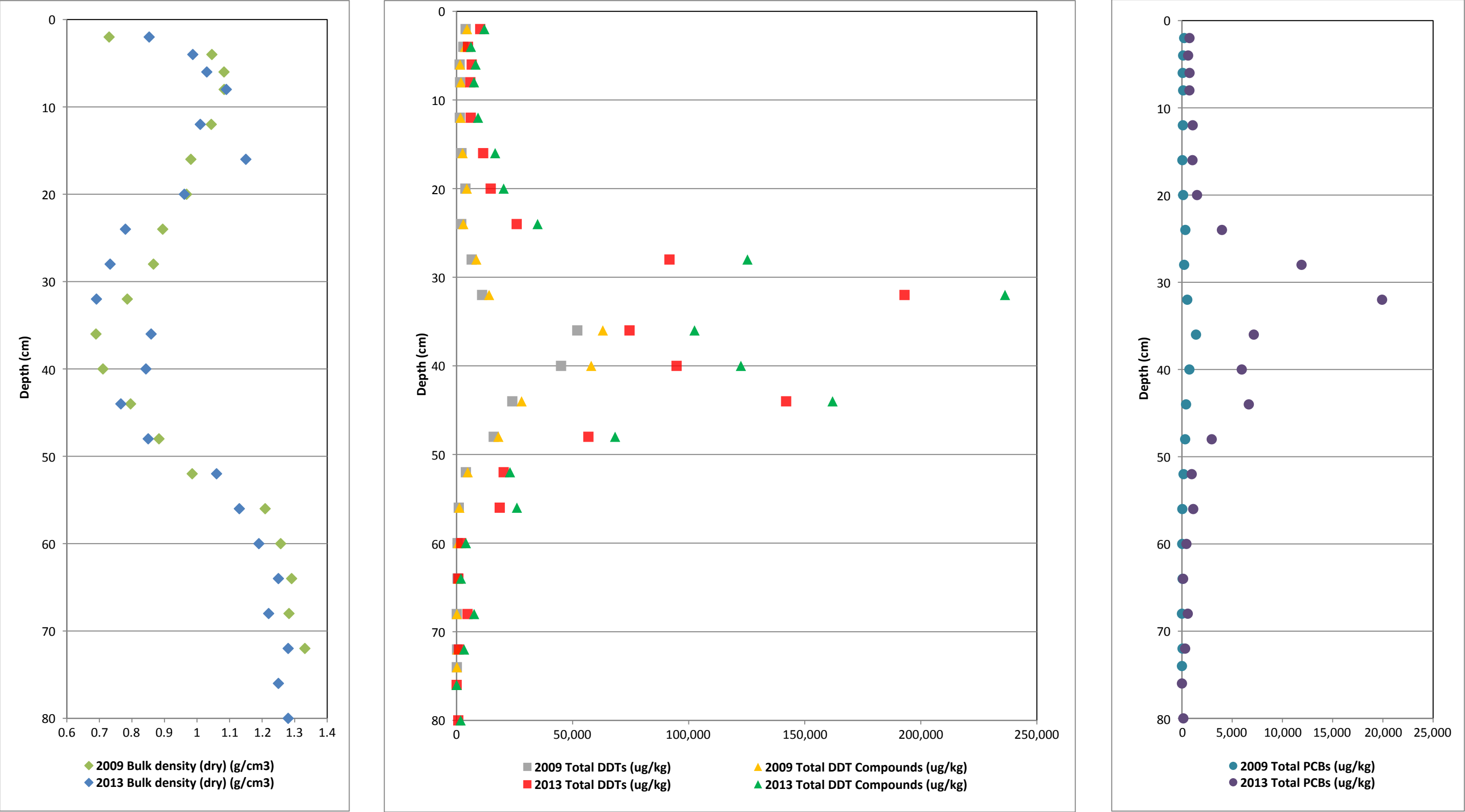
Figure 11. Vertical Profiles of Bulk Density and COCs for Core OA11 First MNR Report Palos Verdes Shelf (OU 5 of the Montrose Chemical Corp. Superfund Site) Los Angeles County, California
