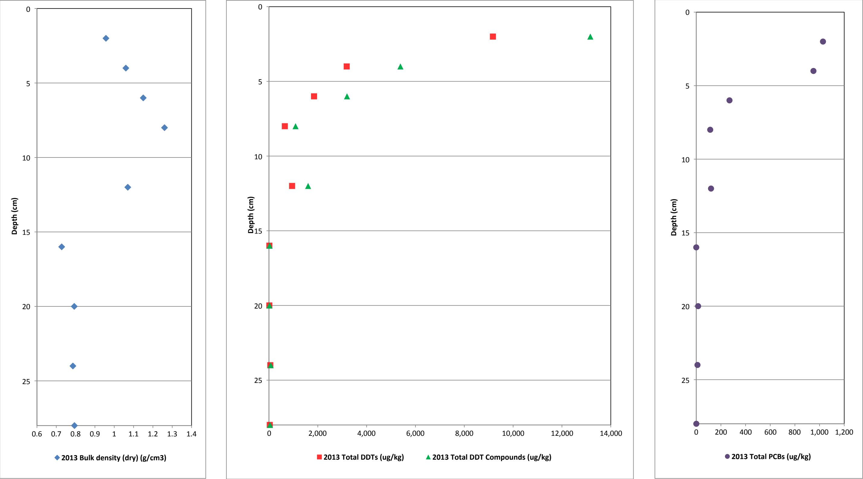
Figure 27. Vertical Profiles of Bulk Density and COCs for Core OA27 First MNR Report Palos Verdes Shelf (OU 5 of the Montrose Chemical Corp. Superfund Site) Los Angeles County, California
