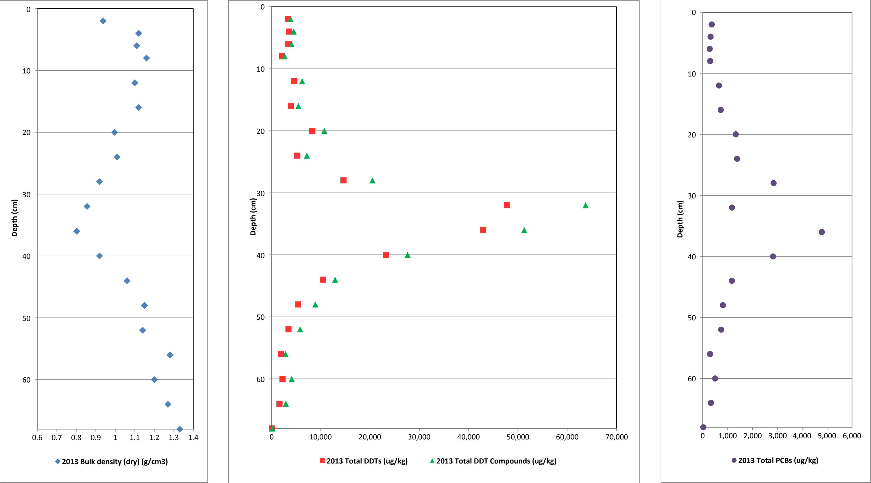
Figure 30. Vertical Profiles of Bulk Density and COCs for Core OA30 First MNR Report Palos Verdes Shelf (OU 5 of the Montrose Chemical Corp. Superfund Site) Los Angeles County, California
