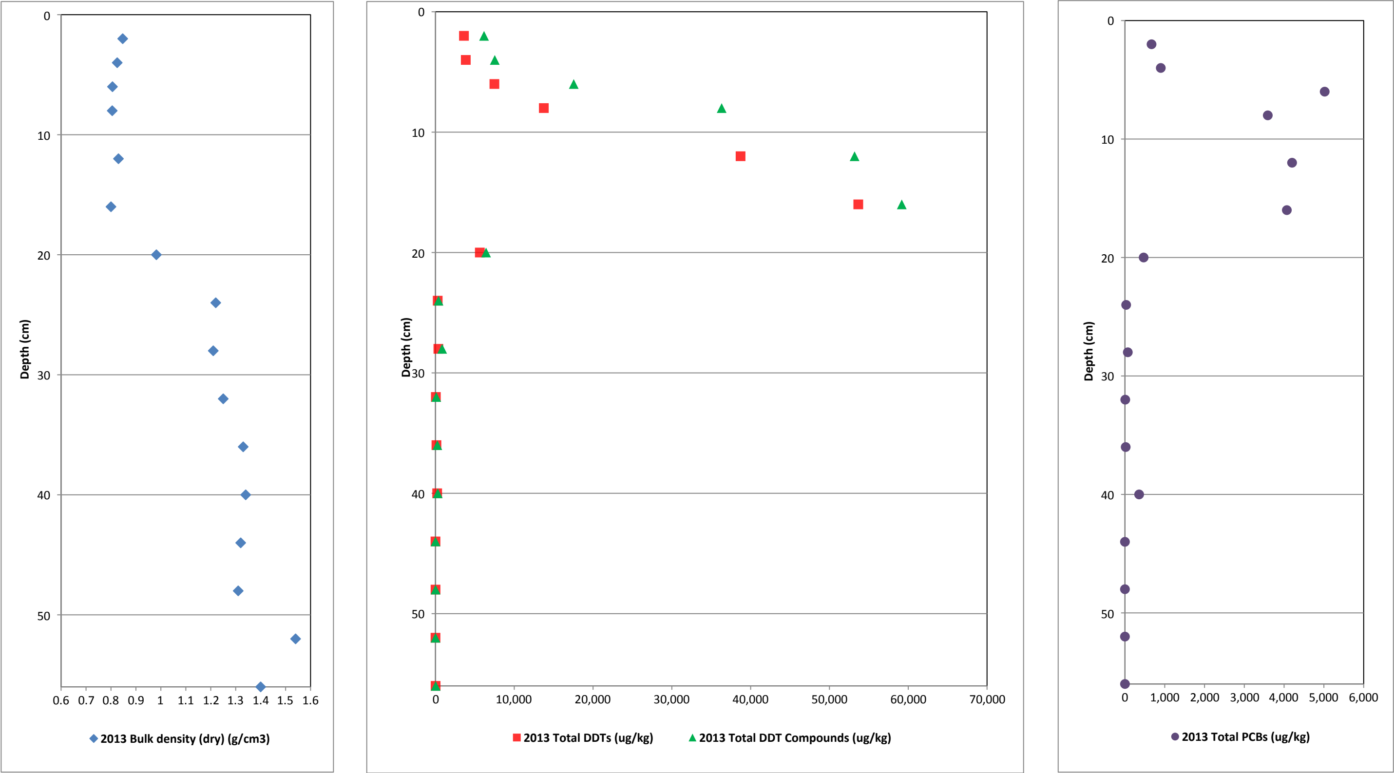
Figure 29. Vertical Profiles of Bulk Density and COCs for Core OA29 First MNR Report Palos Verdes Shelf (OU 5 of the Montrose Chemical Corp. Superfund Site) Los Angeles County, California
