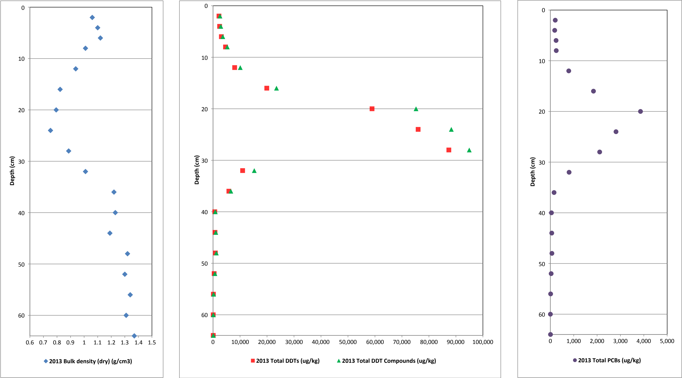
Figure 31. Vertical Profiles of Bulk Density and COCs for Core OA31 First MNR Report Palos Verdes Shelf (OU 5 of the Montrose Chemical Corp. Superfund Site) Los Angeles County, California
