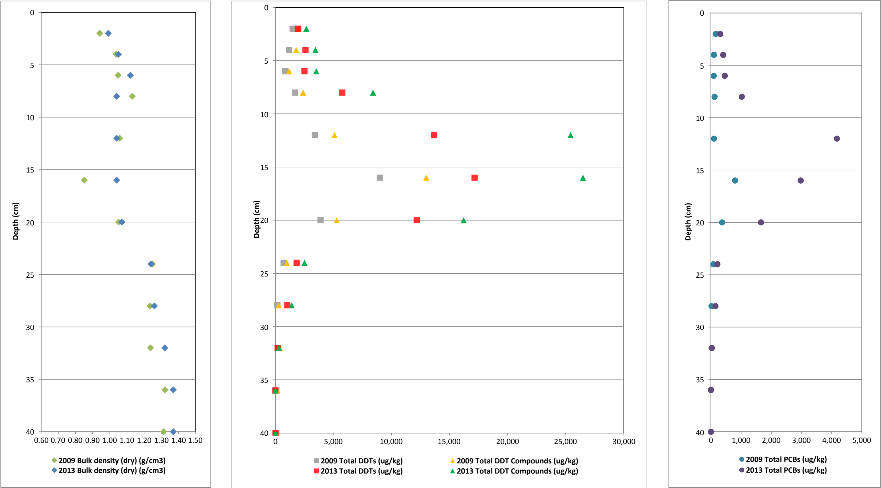
Figure 12. Vertical Profiles of Bulk Density and COCs for Core OA12 First MNR Report Palos Verdes Shelf (OU 5 of the Montrose Chemical Corp. Superfund Site) Los Angeles County, California
