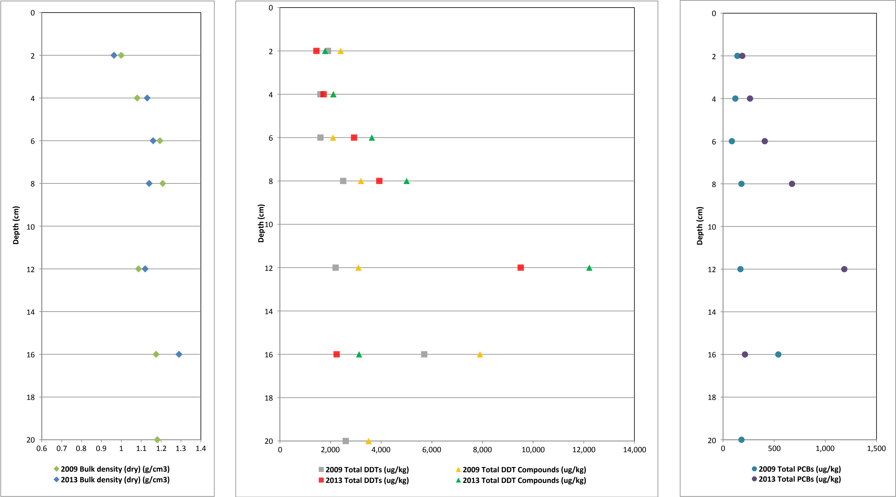
Figure 21. Vertical Profiles of Bulk Density and COCs for Core OA21 First MNR Report Palos Verdes Shelf (OU 5 of the Montrose Chemical Corp. Superfund Site) Los Angeles County, California
