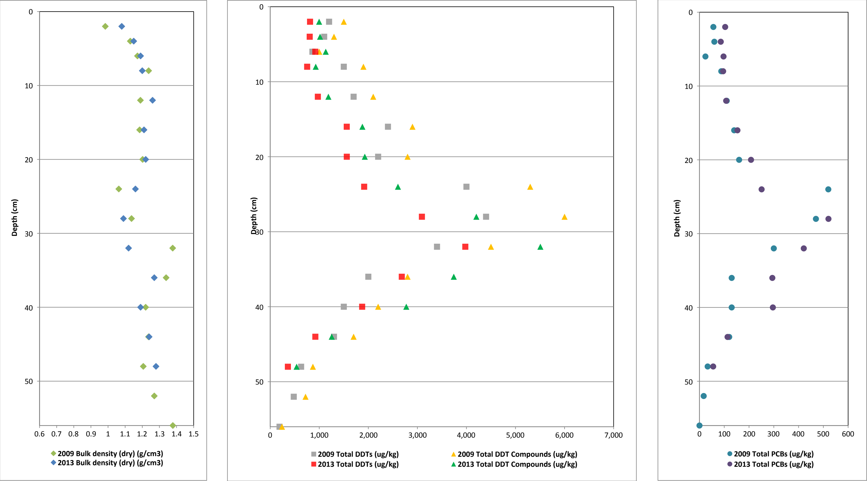
Figure 23. Vertical Profiles of Bulk Density and COCs for Core OA23 First MNR Report Palos Verdes Shelf (OU 5 of the Montrose Chemical Corp. Superfund Site) Los Angeles County, California
