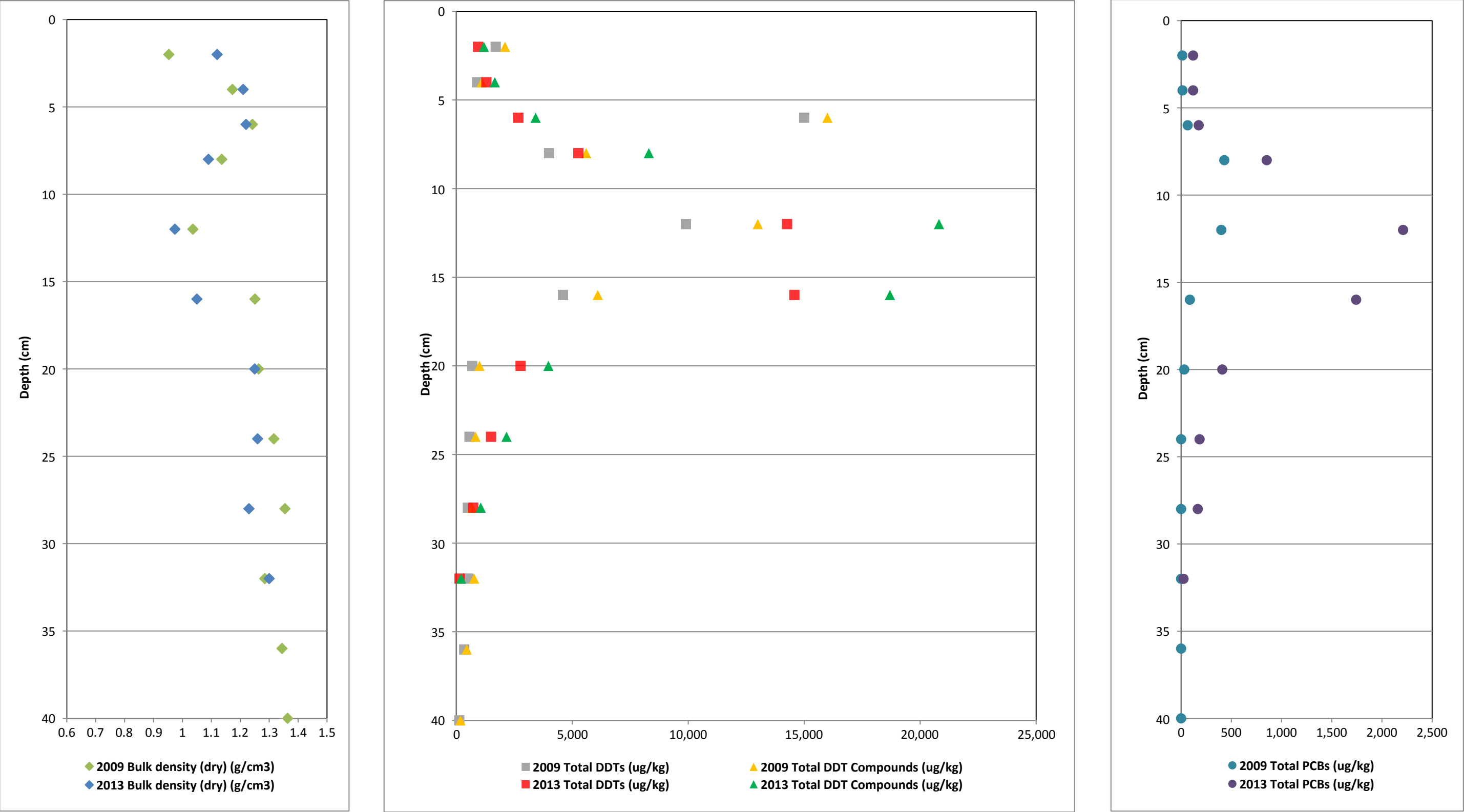
Figure 17. Vertical Profiles of Bulk Density and COCs for Core OA17 First MNR Report Palos Verdes Shelf (OU 5 of the Montrose Chemical Corp. Superfund Site) Los Angeles County, California
