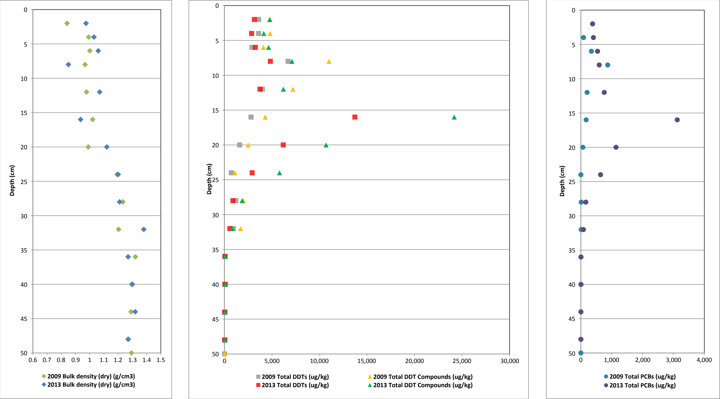
Figure 15. Vertical Profiles of Bulk Density and COCs for Core OA15 First MNR Report Palos Verdes Shelf (OU 5 of the Montrose Chemical Corp. Superfund Site) Los Angeles County, California
