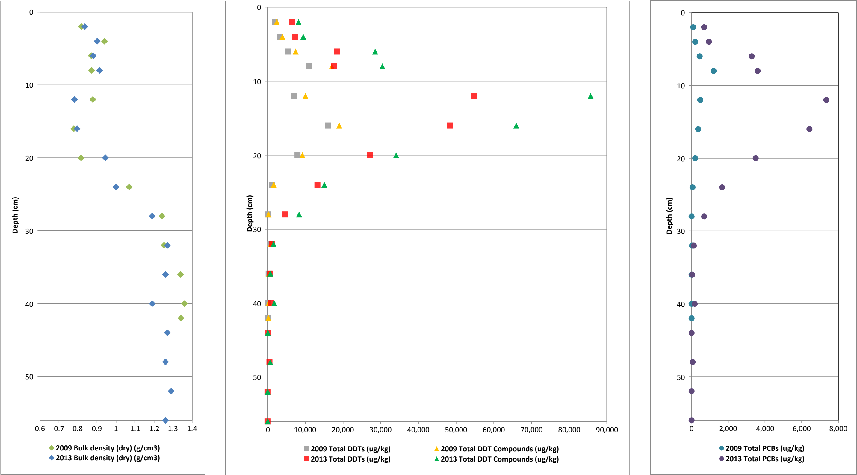
Figure 7. Vertical Profiles of Bulk Density and COCs for Core OA07 First MNR Report Palos Verdes Shelf (OU 5 of the Montrose Chemical Corp. Superfund Site) Los Angeles County, California
