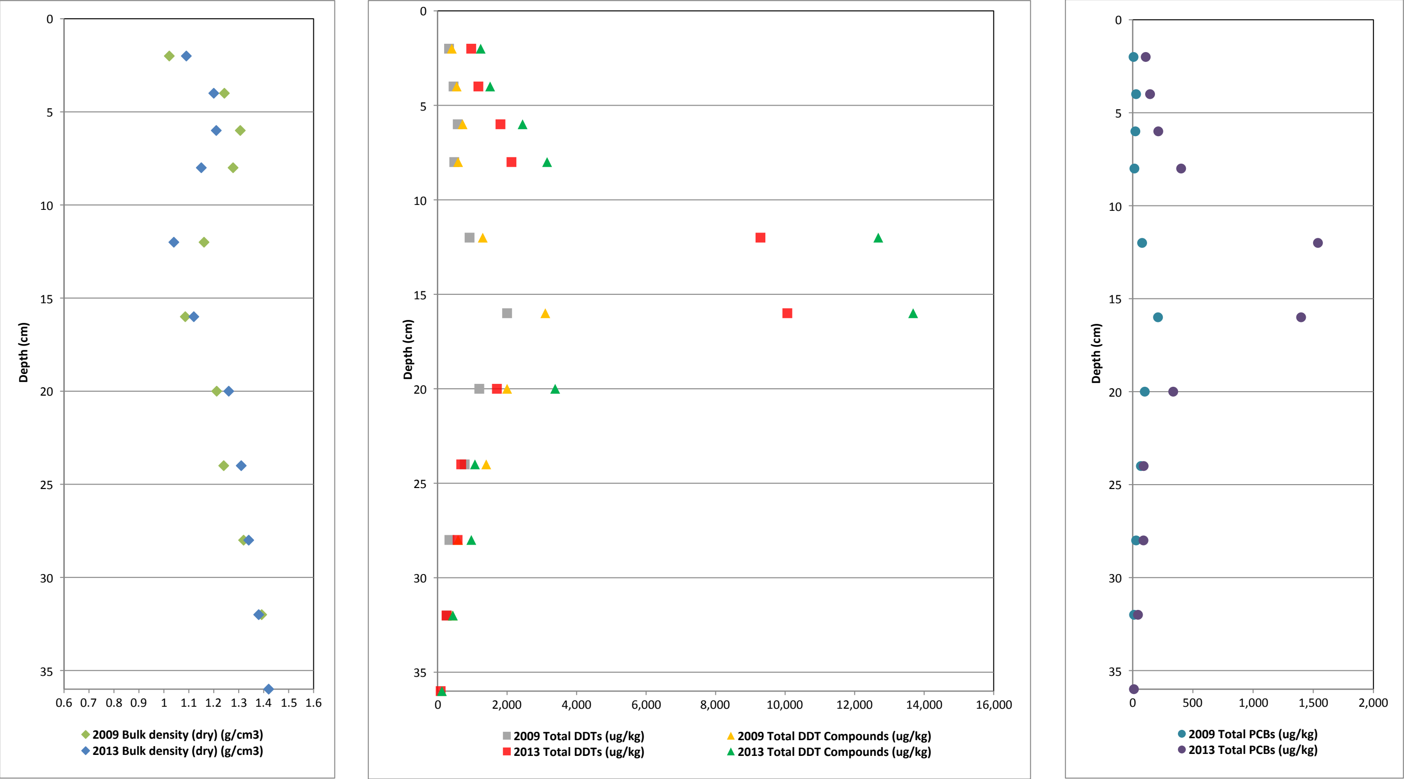
Figure 22. Vertical Profiles of Bulk Density and COCs for Core OA22 First MNR Report Palos Verdes Shelf (OU 5 of the Montrose Chemical Corp. Superfund Site) Los Angeles County, California
