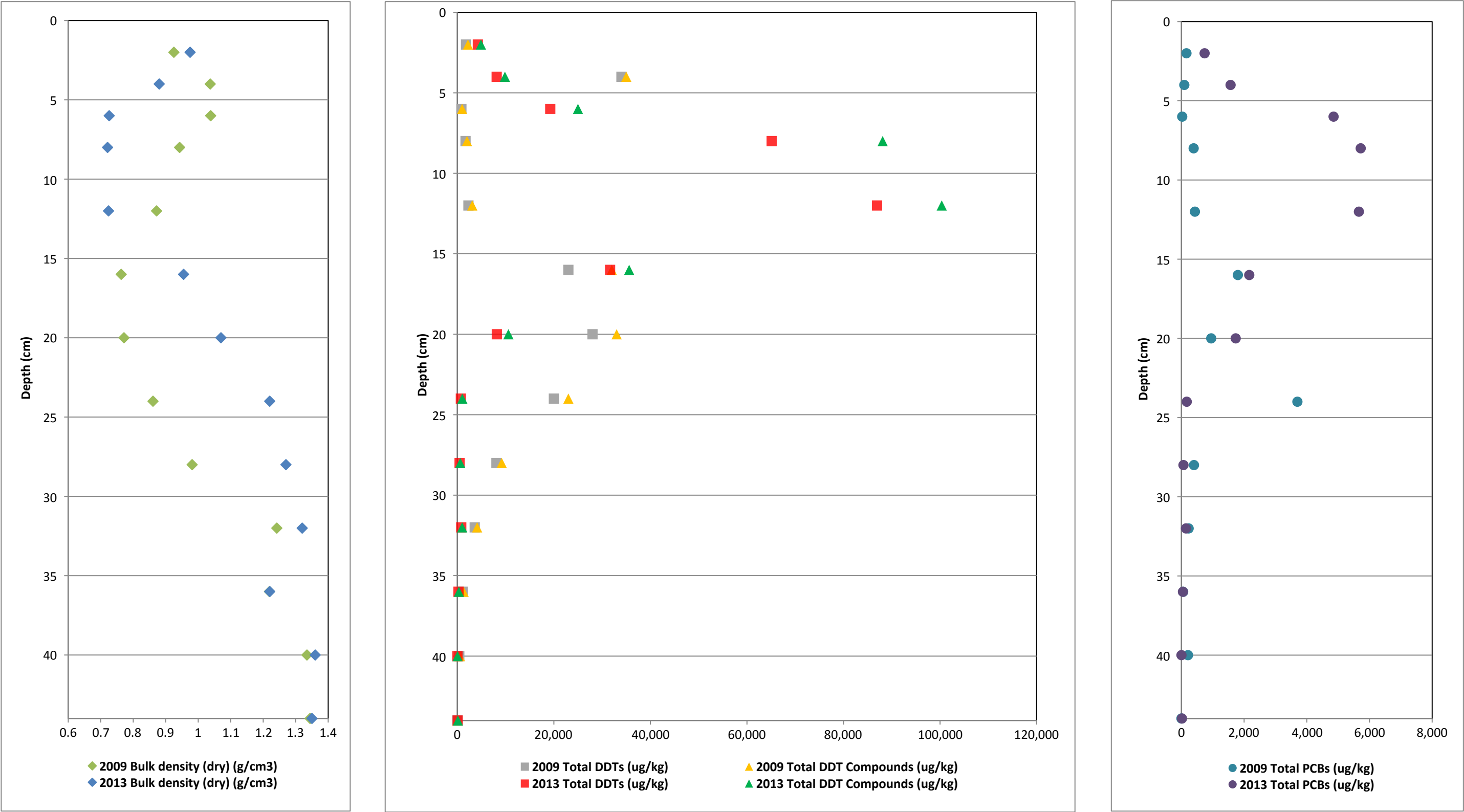
Figure 4. Vertical Profiles of Bulk Density and COCs for Core OA04 First MNR Report Palos Verdes Shelf (OU 5 of the Montrose Chemical Corp. Superfund Site) Los Angeles County, California
