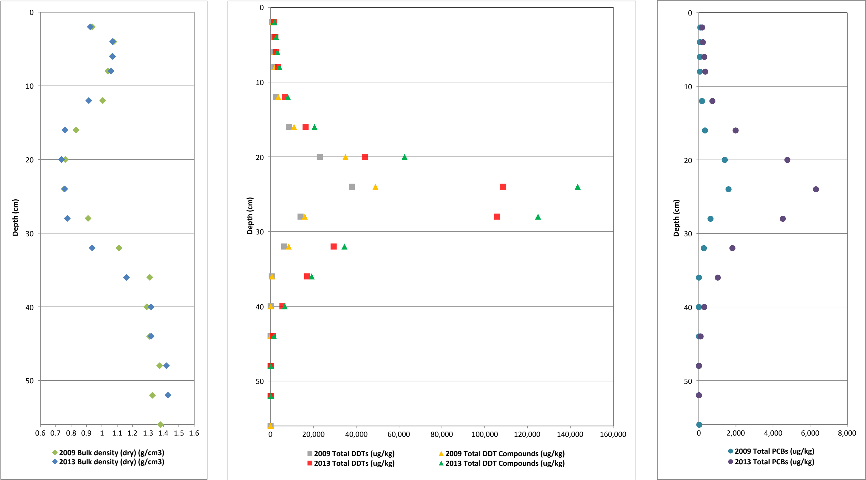
Figure 1. Vertical Profiles of Bulk Density and COCs for Core OA01 First MNR Report Palos Verdes Shelf (OU 5 of the Montrose Chemical Corp. Superfund Site) Los Angeles County, California
