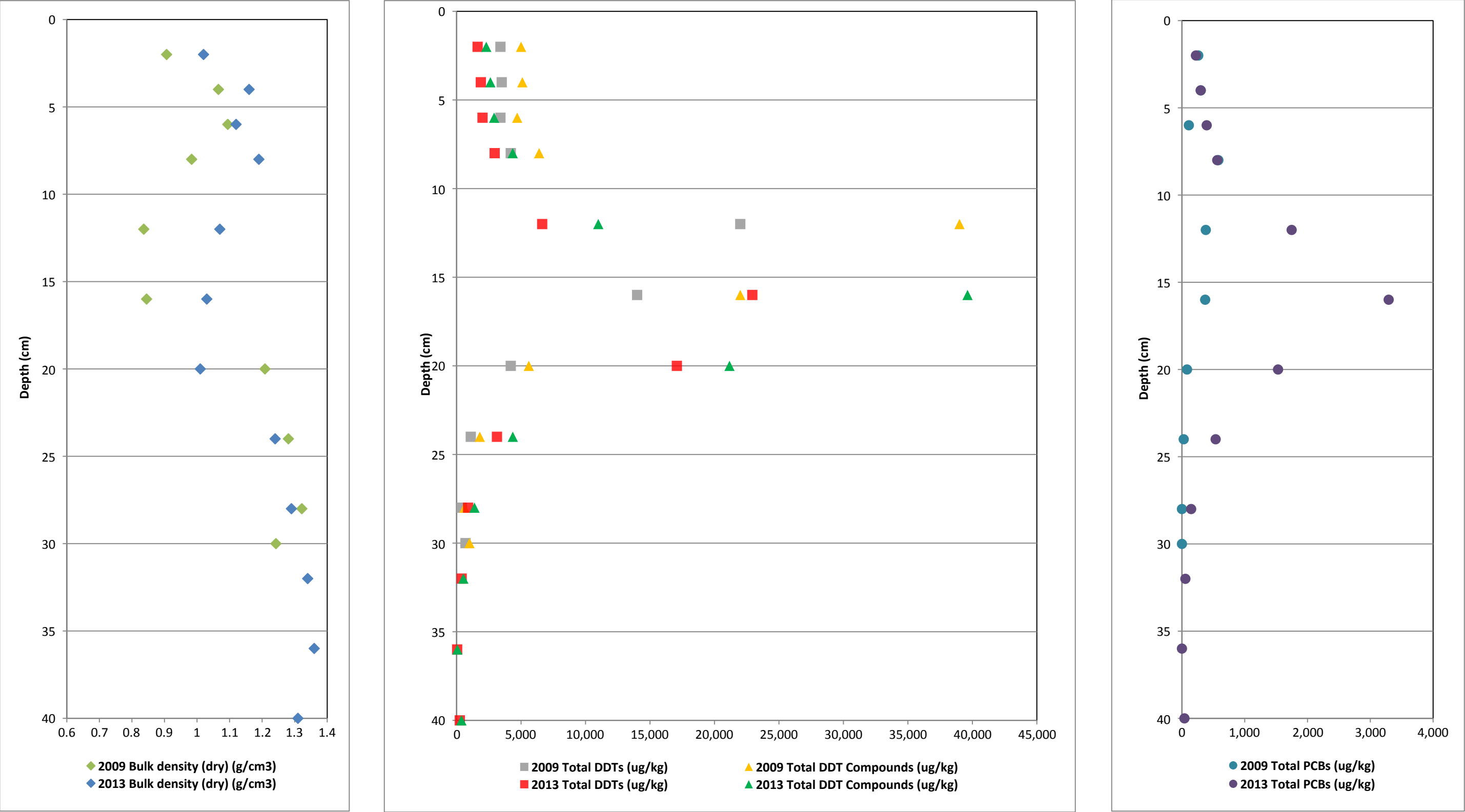
Figure 16. Vertical Profiles of Bulk Density and COCs for Core OA16 First MNR Report Palos Verdes Shelf (OU 5 of the Montrose Chemical Corp. Superfund Site) Los Angeles County, California
