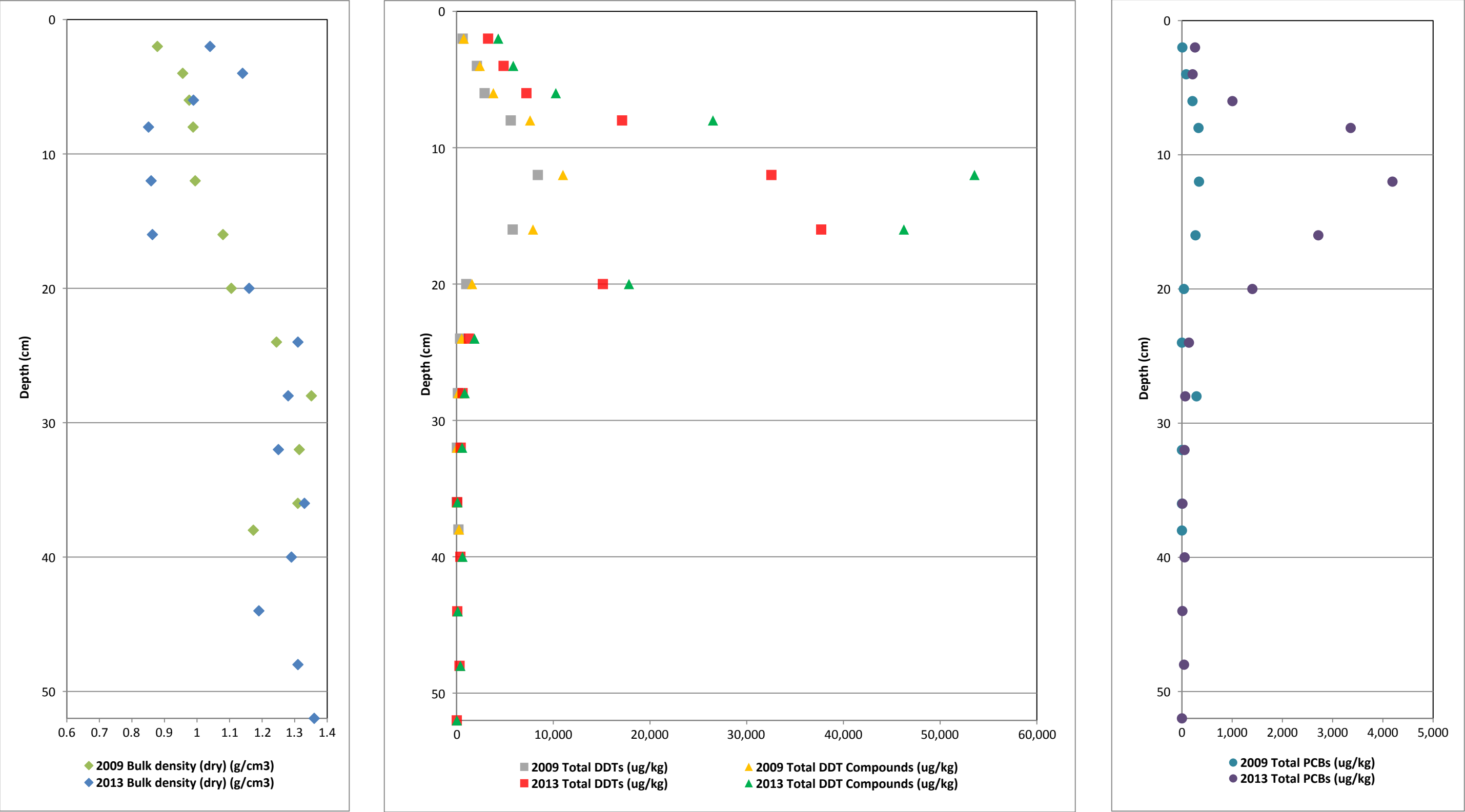
Figure 10. Vertical Profiles of Bulk Density and COCs for Core OA10 First MNR Report Palos Verdes Shelf (OU 5 of the Montrose Chemical Corp. Superfund Site) Los Angeles County, California
